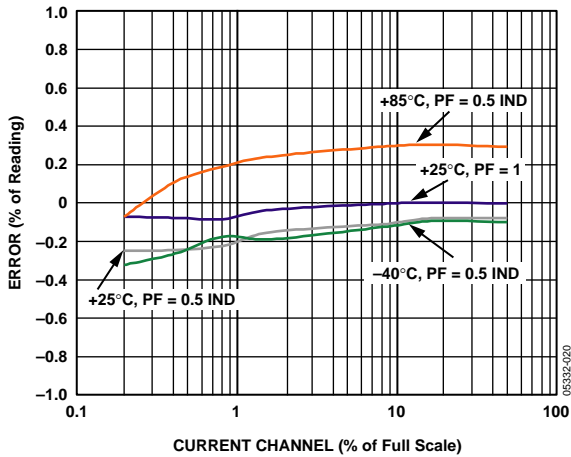
Figure 6. Error as a % of Reading over Temperature with On-Chip Reference (PF = 0.5)
